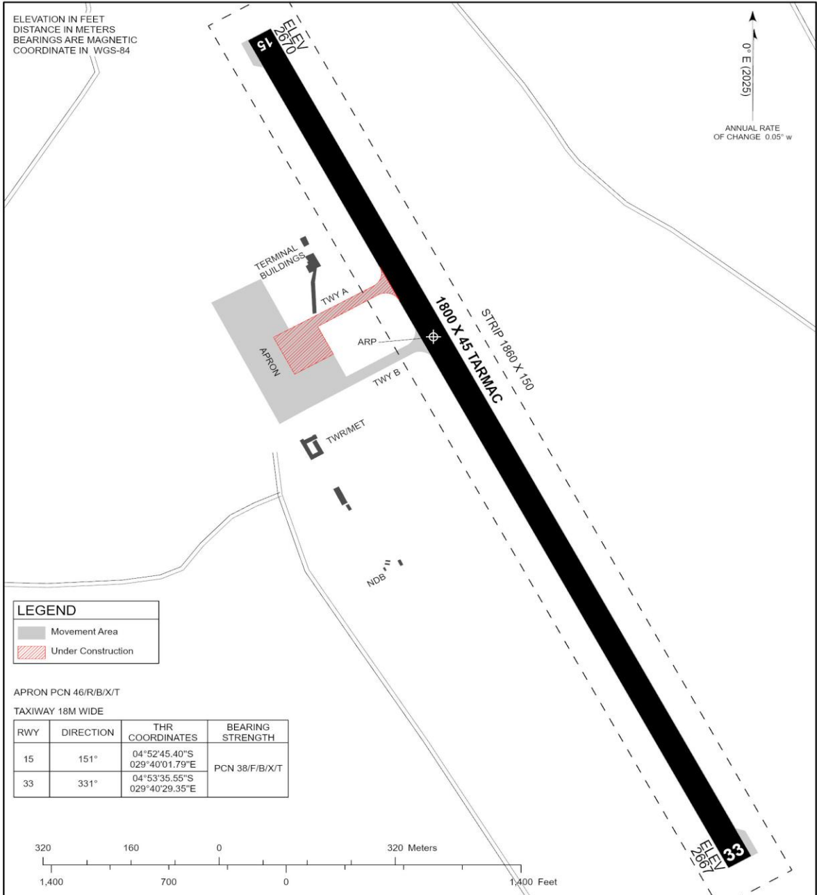
MARKINGS AIDS RWY 15/33 AND ENTRY/EXIT TWY
